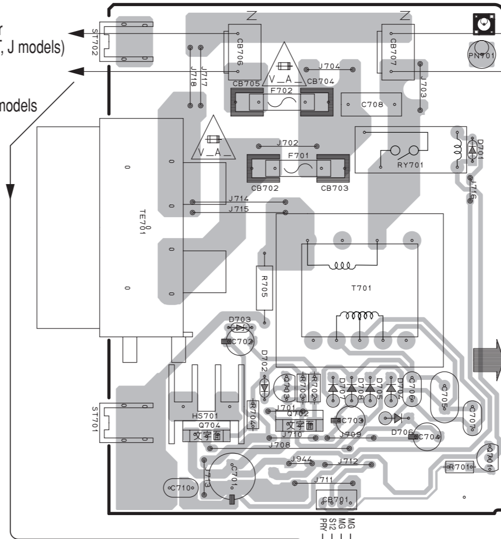
POWER (3) P. C. B. (Lead Type Device)
