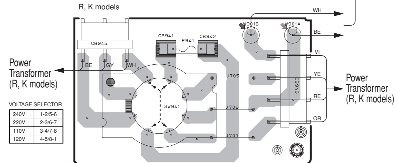
POWER (3) P. C. B. (Lead Type Device)
